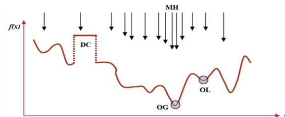
Figure 3: Simplified representation of a metaheuristic approach [23]
