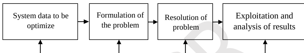
Figure 1: Steps to solve an optimization problem
