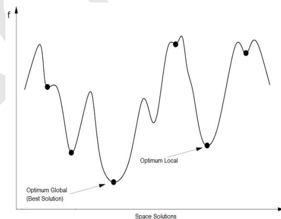
Figure 2: Local minimum and global minimum
